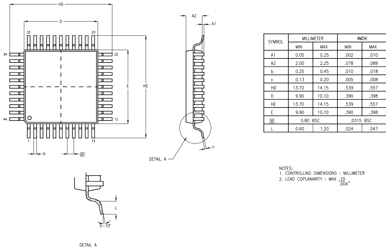
Figure 24. 44-Lead Plastic Quad Flat Pack
